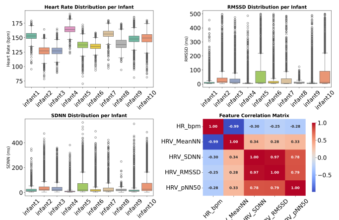
Fig. 3. Exploratory analysis of ECG-derived HRV features extracted from the PICS dataset. Box plots show inter-subject variability in heart rate, RMSSD, and SDNN across 10 infants, alongside the feature correlation matrix.
